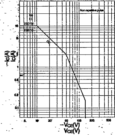
Area of Safe Operation (ASO) ( T_c = 25^\circ\text{C} )
