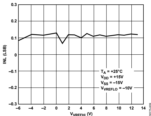
Figure 8. INL vs. V_{VREFHI} ( \pm 15\text{ V} )
