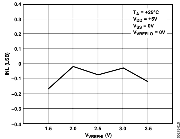
Figure 9. INL vs. V_{VREFHI} ( +5\text{ V} )
