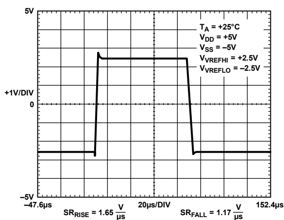
Figure 23. Slew Rate ( \pm 5\text{ V} )
