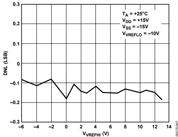
Figure 6. DNL vs. V_{VREFHI} ( \pm 15\text{ V} )
