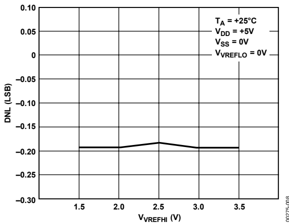
Figure 7. DNL vs. V_{VREFHI} ( +5\text{ V} )
