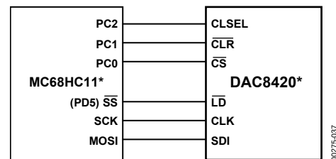
Figure 37. MC68HC11 Microcontroller Interface
