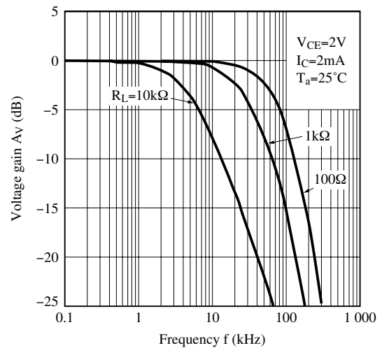
Fig.15 Frequency Response
