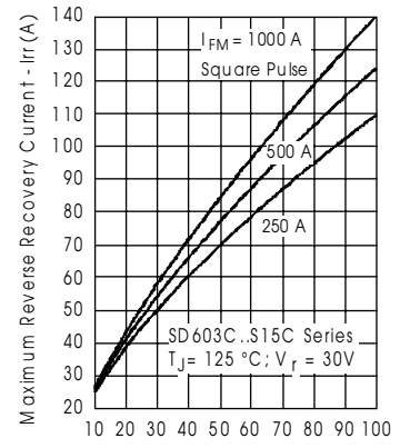
Fig. 17 - Recovery Current Characteristics
