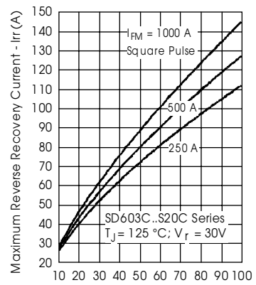
Fig. 20 - Recovery Current Characteristics
