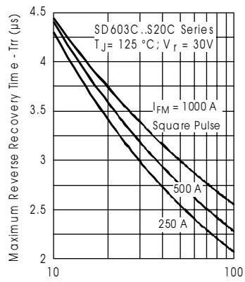
Fig. 18 - Recovery Time Characteristics
