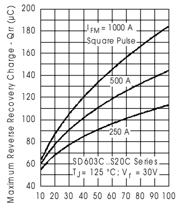
Fig. 19 - Recovery Charge Characteristics
