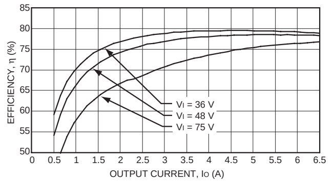
Figure 4. JBW030F Typical Converter Efficiency vs. Output Current
