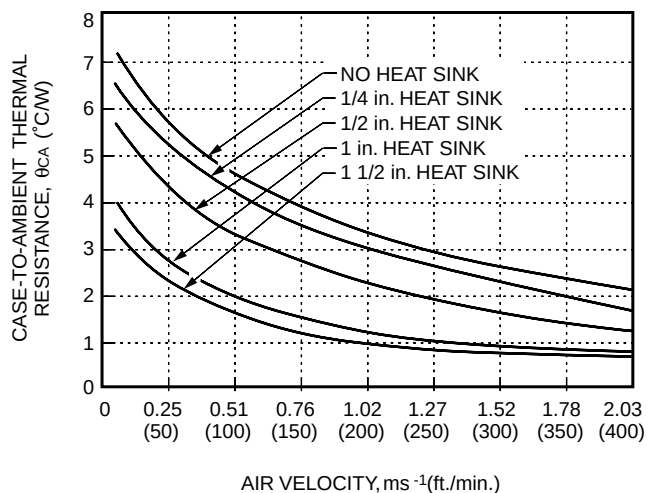
Figure 22. Case-to-Ambient Thermal Resistance vs. Air Velocity Curves; Either Orientation
