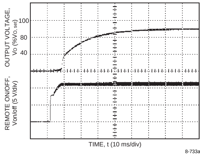
Figure 10. Typical Output Voltage Start-Up when Signal Applied to Remote On/Off
