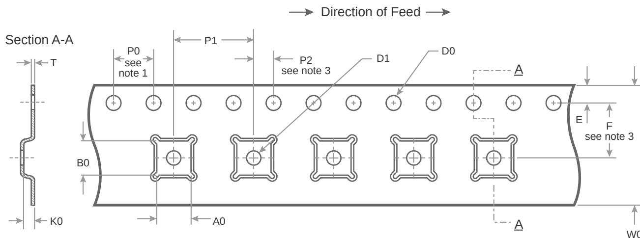
Figure 28 • Tape and Reel Specifications for 20-lead 4 \times 4 \times 0.85 mm QFN
