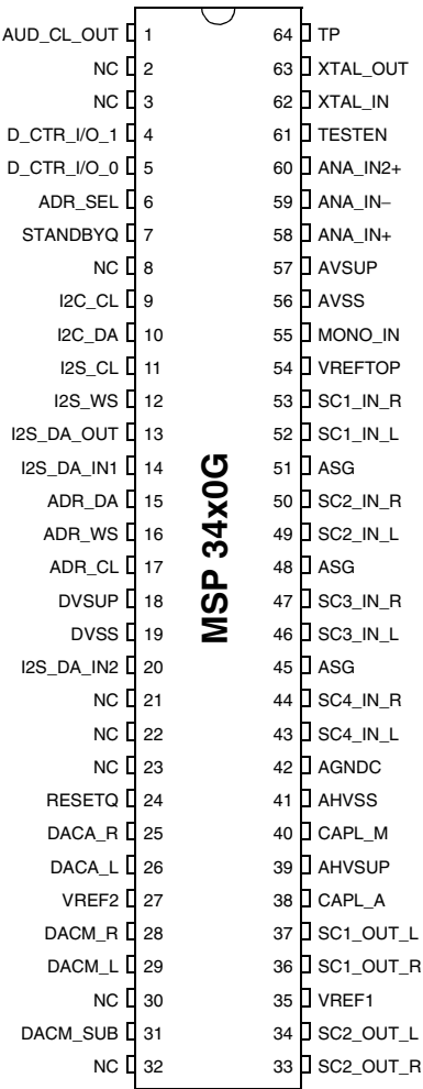
Fig. 4-6: PSDIP64-1 package
