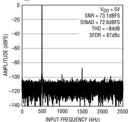
16k point FFT f_S = 5\text{MSPS} f_{IN} = 500\text{kHz}
