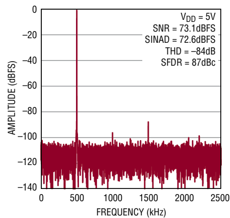
f S = 5Mps, f IN = 500kHz 16k-pt FFT
