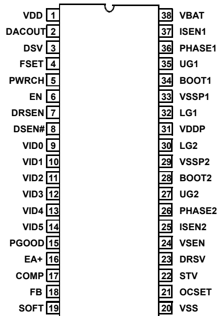
ISL9500 (38 LD TSSOP) TOP VIEW
