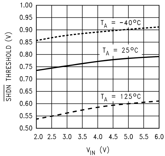
\overline{SHDN} Threshold vs V_{IN}
