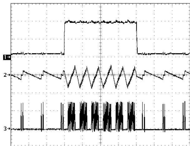
Step Response
