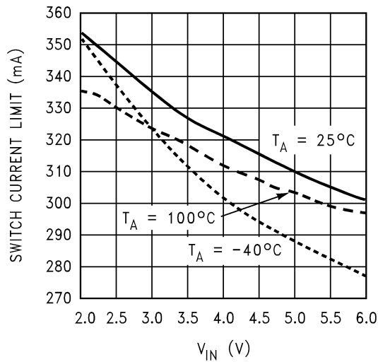
Switch Current Limit vs V_{IN}
