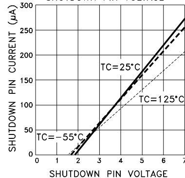
SHUTDOWN PIN CURRENT vs. SHUTDOWN PIN VOLTAGE
