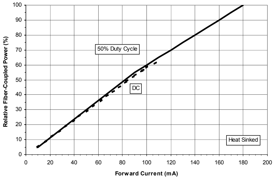
Figure 5 - Relative Fiber-coupled Power vs. Forward Current
