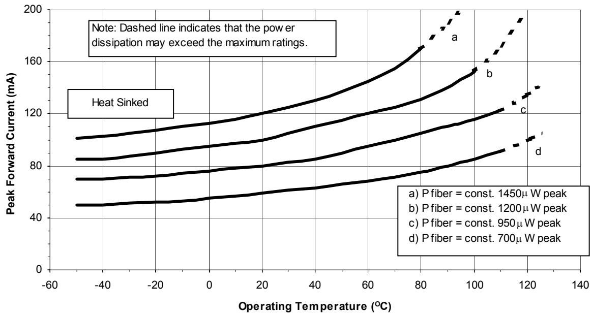
Figure 8 - Peak Forward Current vs. Operating Temperature
