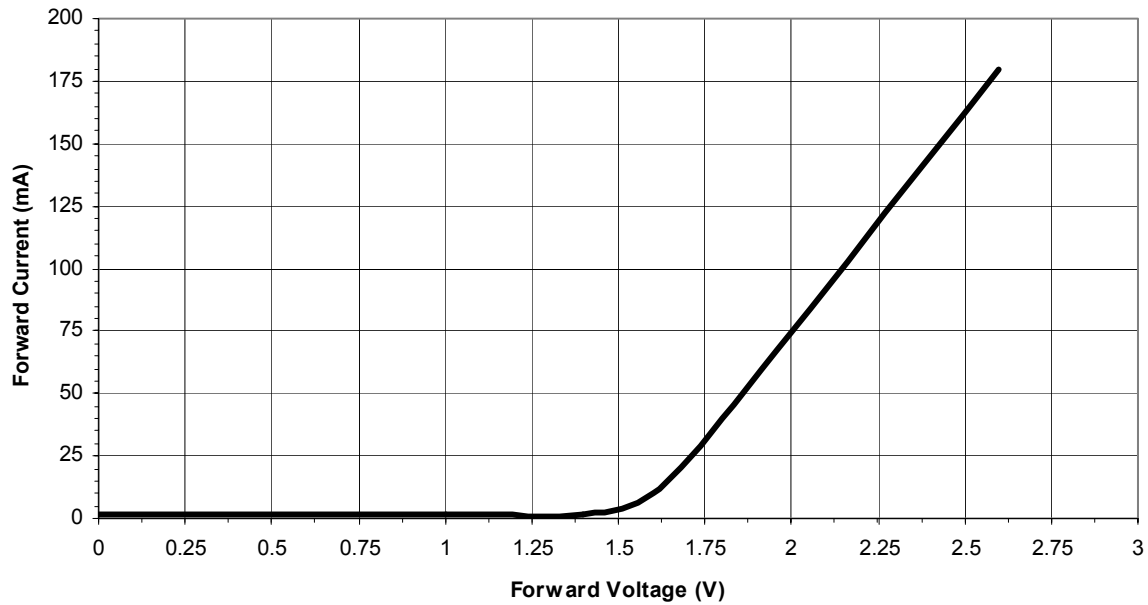
Figure 7 - Forward Current vs. Forward Voltage
