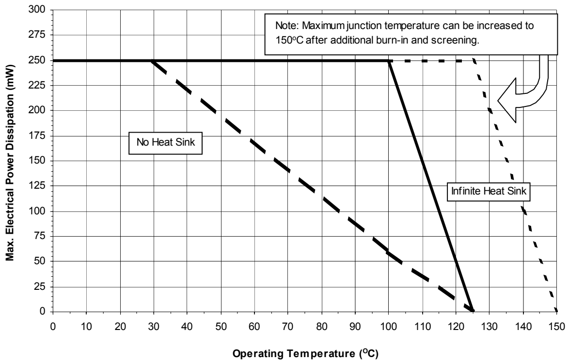
Figure 6 - Max. Electrical Power Dissipation vs. Operating Temperature
