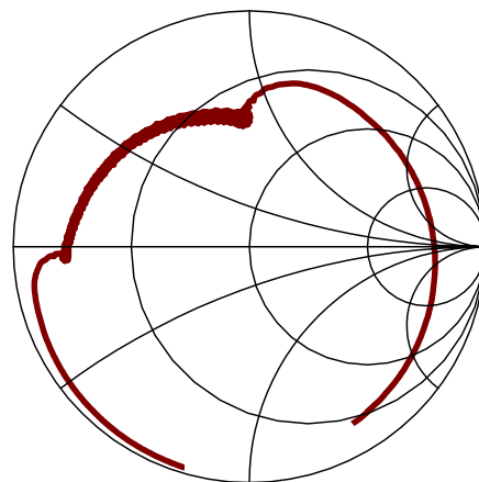
S22 (60-180 MHz)
