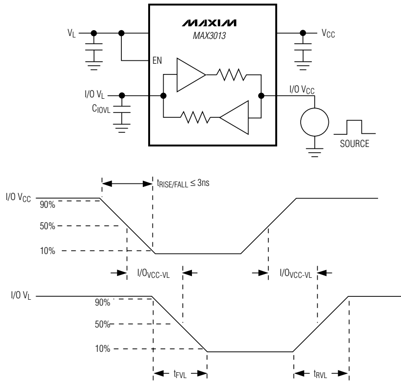
Figure 2. Driving I/O V_{CC} Test Circuit and Timing
