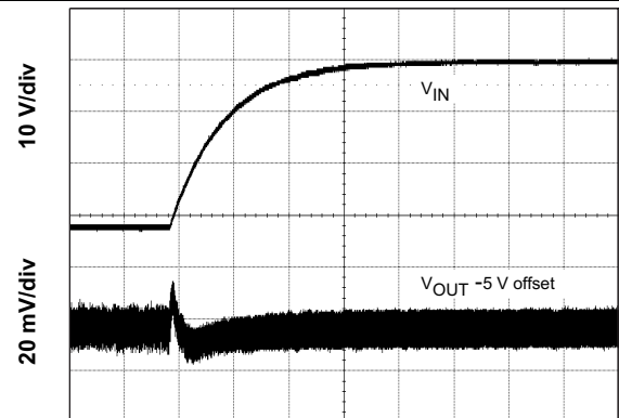
Time = 5 ms/div Figure 35. Line Transient (8 V To 40 V)
