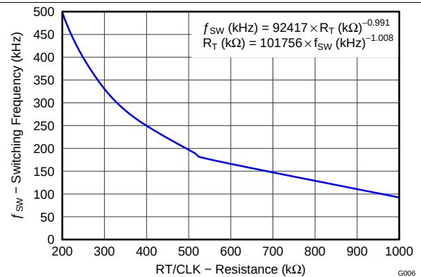
Figure 6. Switching Frequency vs R_T/\text{CLK} Resistance Low Frequency Range
