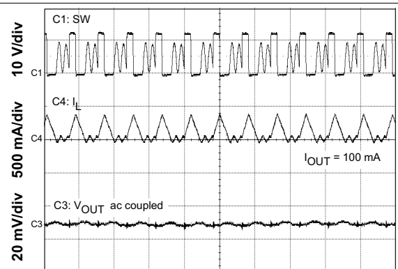
Time = 2 \mu s/div Figure 39. Output Ripple DCM
