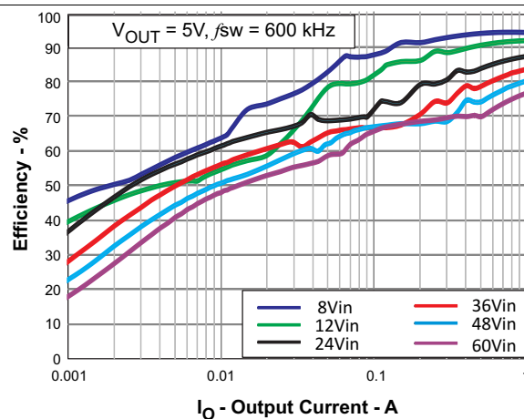
Figure 45. Light Load Efficiency
