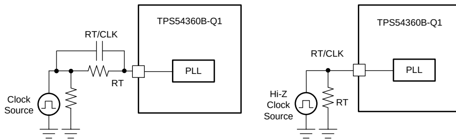
Figure 25. Synchronizing to a System Clock
