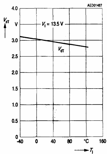
Delay Switching Threshold V_{dT} versus Temperature T_i
