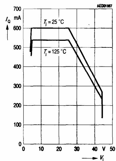
Output Current I_o versus Input Voltage V_i
