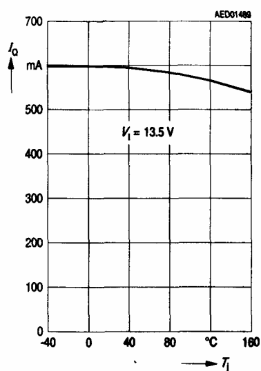
Output Current I_o versus Temperature T_i
