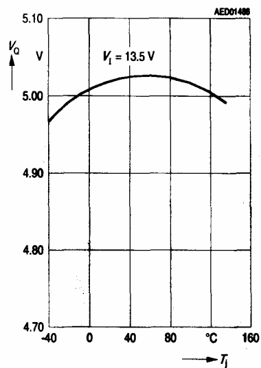
Output Voltage V_o versus Temperature T_i
