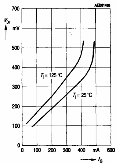
Drop Voltage V_{Dr} versus Output Current I_o
