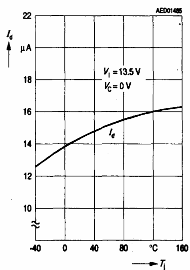
Charge Current I_d versus Temperature T_i
