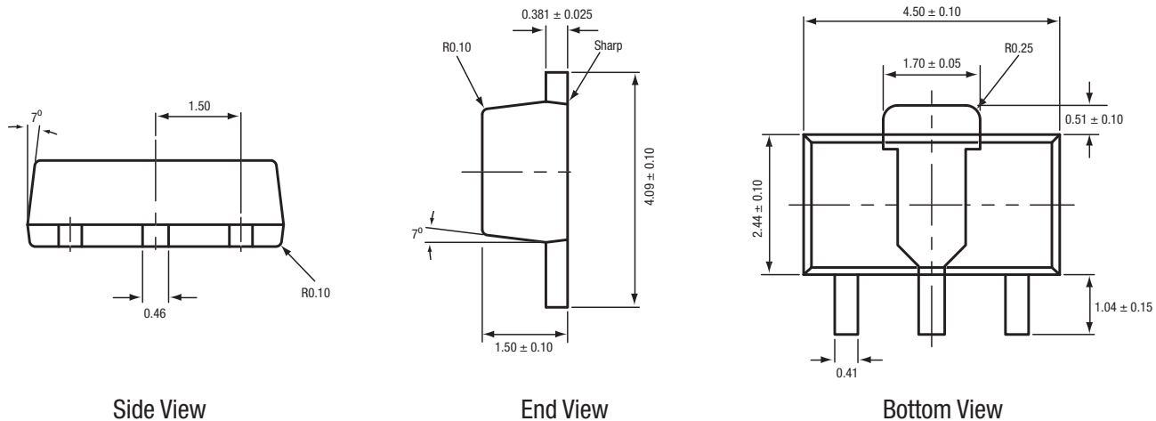
Figure 13. SKY65080-70LF (4-Pin SOT-89) Package Dimensions
