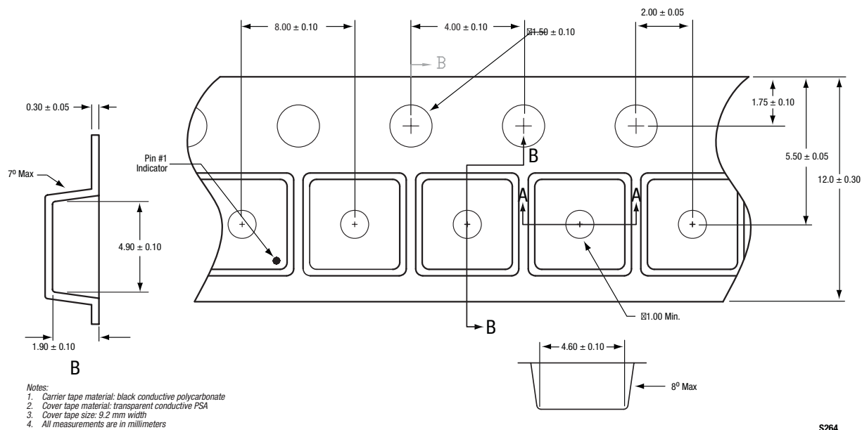
Figure 14. SKY65080-70LF Tape and Reel Dimensions
