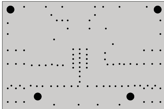
Layer 3: Ground
