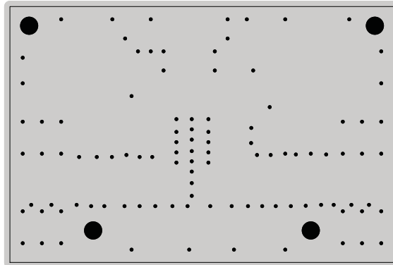
Layer 2: Ground
