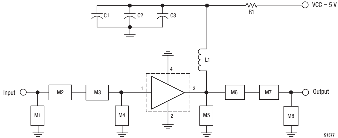
Figure 12. SKY65080-70LF Evaluation Board Schematic (1700 MHz to 2000 MHz, IIP3 Matched)
