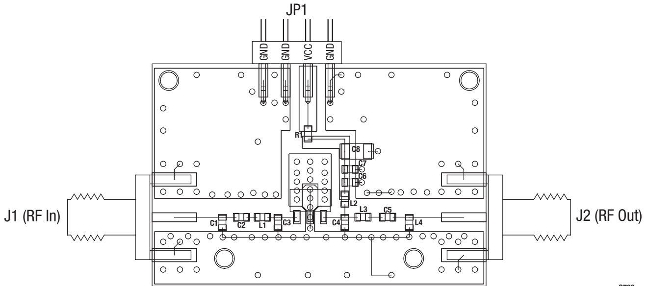
Figure 10. Evaluation Board Assembly Drawing
