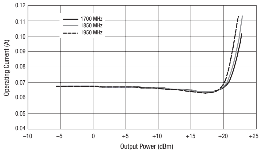
Figure 9. Operating Current vs Output Power Over Frequency
