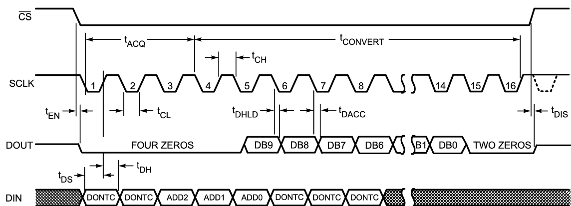
FIGURE 2. ADC108S102 Serial Timing Diagram
