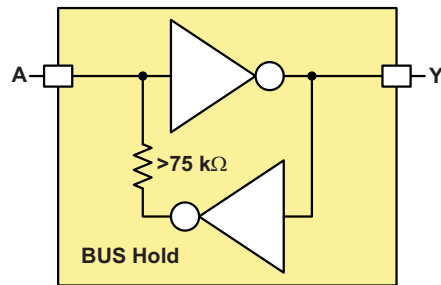
Figure 26. Bus-Hold Circuit
