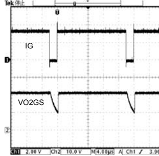
Fig. 24 Gate Shading Output Waveform
