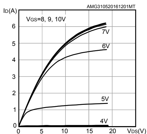
Figure 5. Output characteristics
