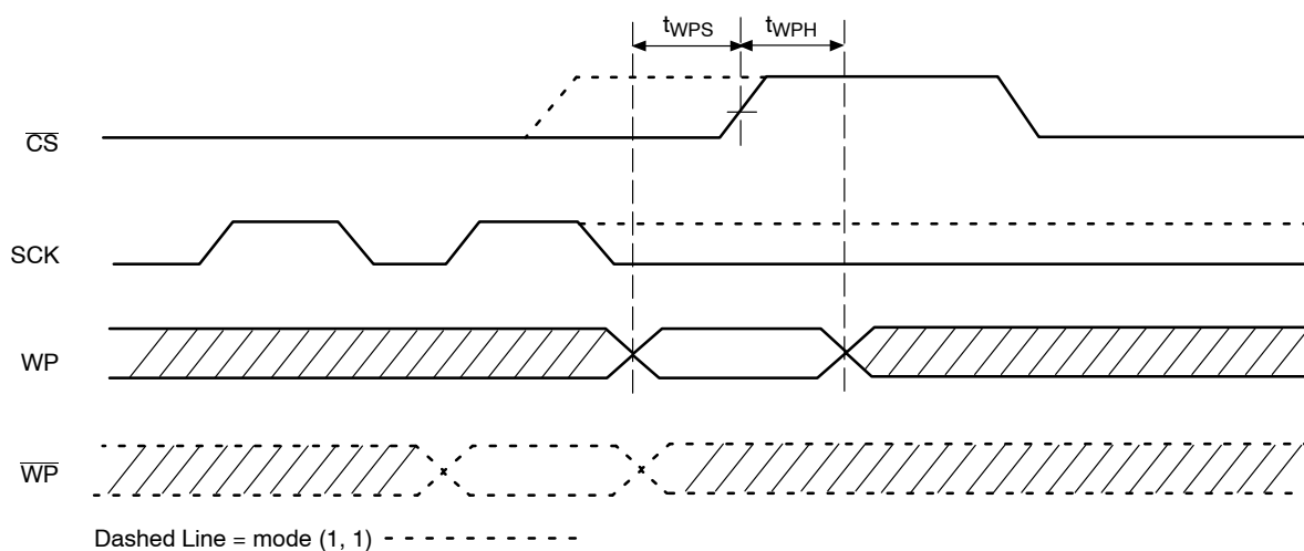
Figure 8. \overline{WP} Timing
