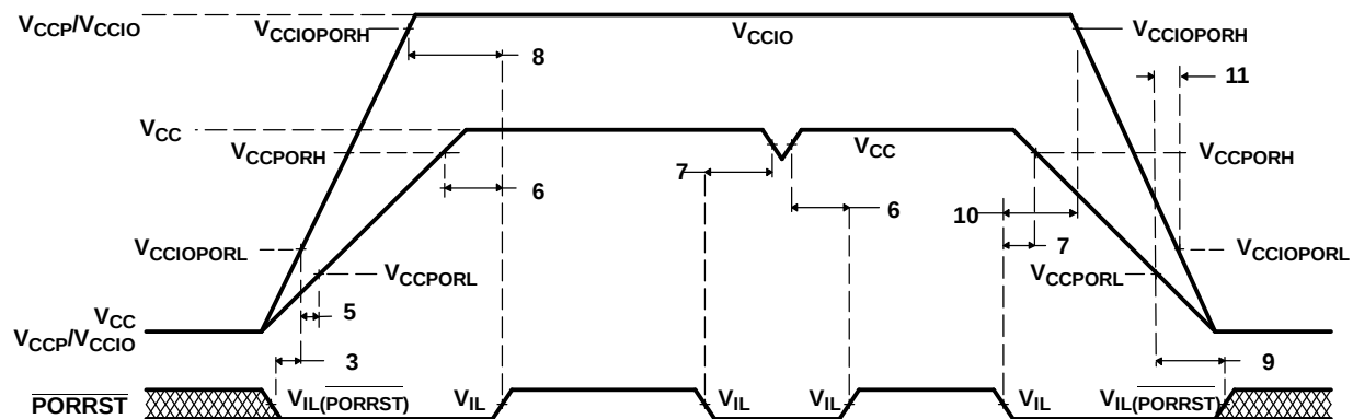
Figure 8. \overline{\text{PORRST}} Timing Diagram
