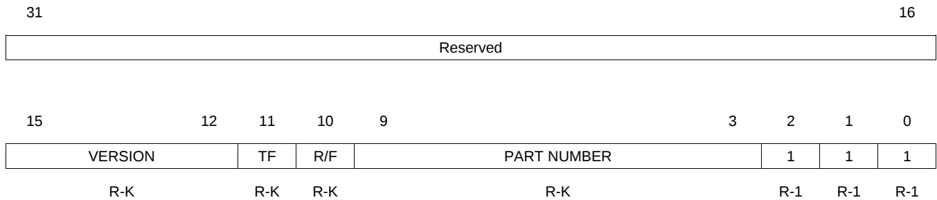
Figure 3. TMS470 Device ID Bit Allocation Register
