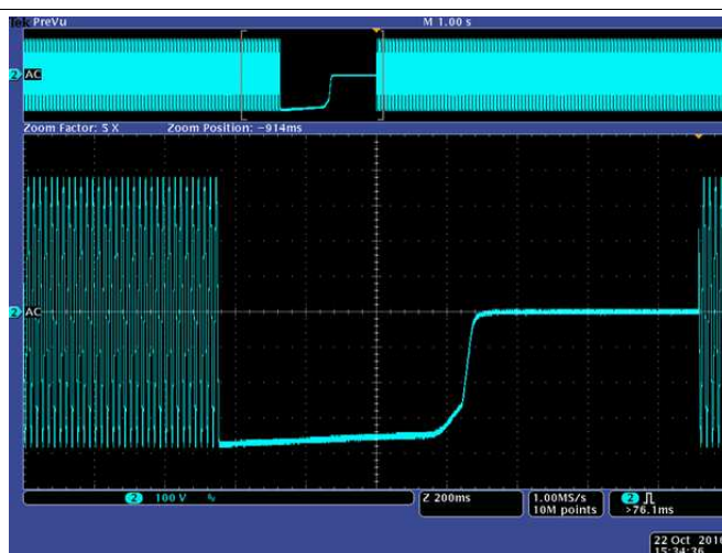
Figure 61. X-Capacitor Discharge
