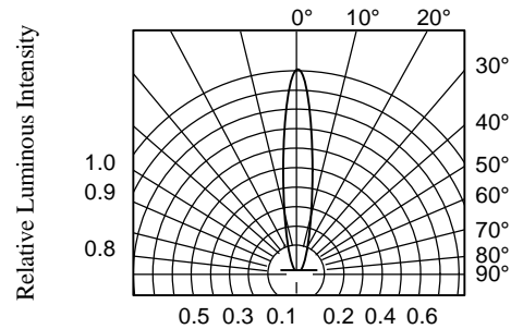
FIG.6 RADIATION DIAGRAM
