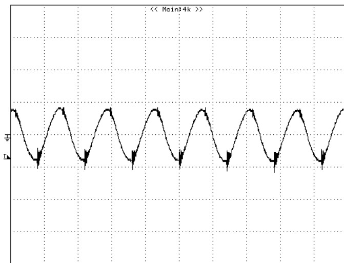
Figure 14: Output voltage ripple at nominal input voltage and rated load current ( I_o=1.5\text{A} ) ( 50\text{mV/div} , 2\mu\text{s/div} ) Load capacitance: 1\mu\text{F} ceramic capacitor and 220\mu\text{F} electrolytic capacitor. Bandwidth: 20\text{MHz} . Scope measurements should be made using a BNC cable (length shorter than 20 inches). Position the load between 51 mm to 76 mm (2 inches to 3 inches) from the module.
