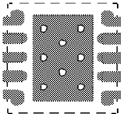
FIGURE 18. PCB VIA PATTERN
