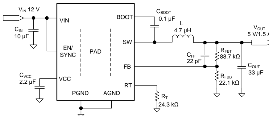
Figure 22. Application Circuit
