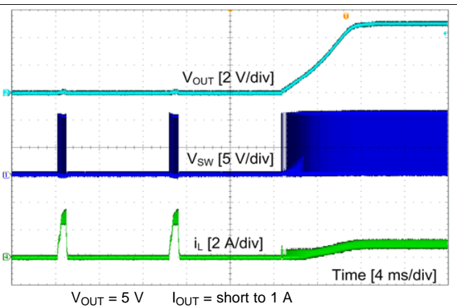
Figure 30. Short Recovery
