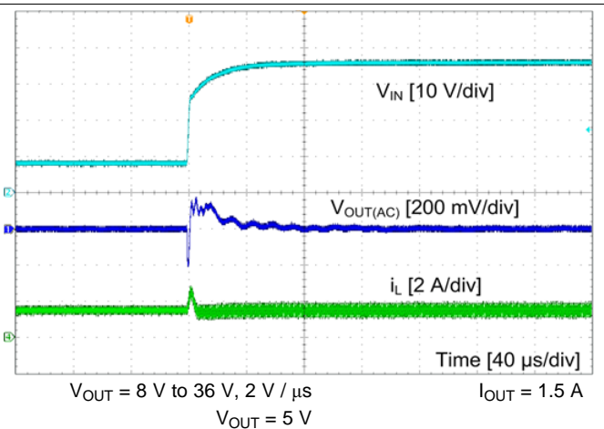
Figure 28. Line Transient
