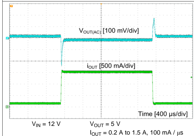
Figure 27. Load Transient
