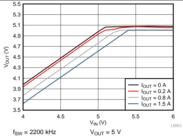
Figure 8. Dropout Curve
