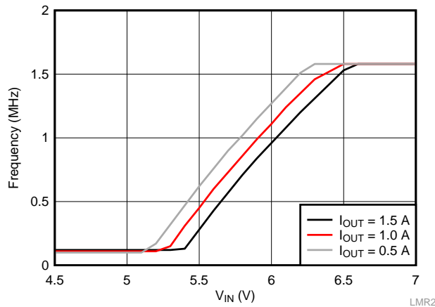
Figure 20. Frequency Foldback at Dropout ( V_{OUT} = 5\text{ V} , f_{SW} = 1600\text{ kHz} )
