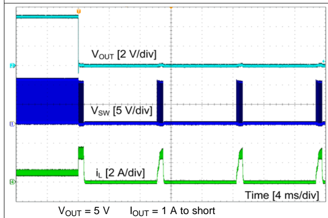
Figure 29. Short Protection
