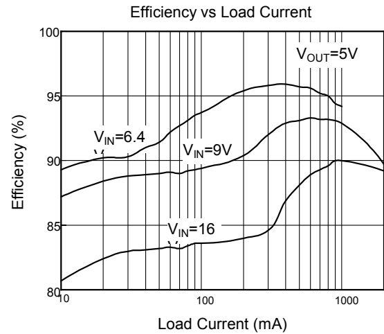
Fig. 1 5V Step-Down Converter
