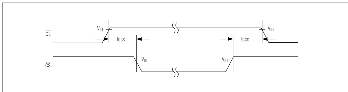
Figure 4. SRAM/RTC Data Bus Control
