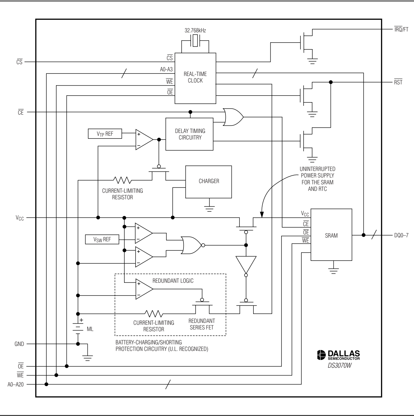
Functional Diagram
