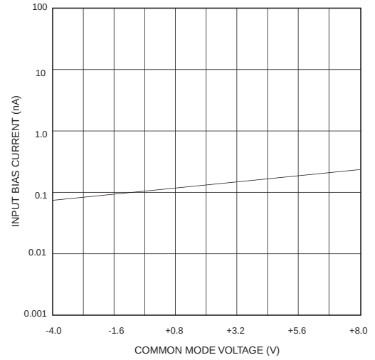
INPUT BIAS CURRENT VS COMMON MODE VOLTAGE ( +25^{\circ}\text{C} )
