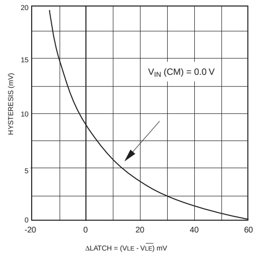
HYSTERESIS VS \Delta\text{LATCH}
