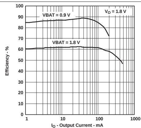
Figure 2. TPS61020 Efficiency vs Output Current
