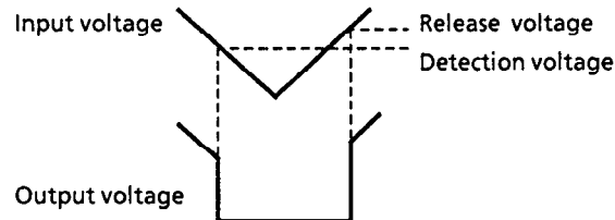
Figure 7 Detection potentials of voltage detectors
