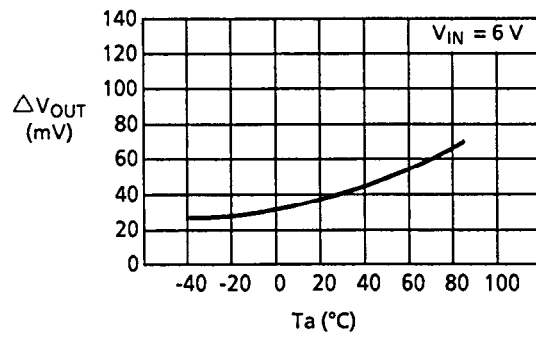
2.14 Load stability ( V_{OUT} ) - Temperature
