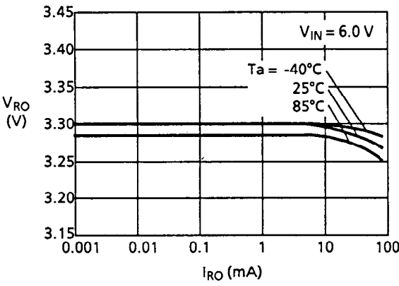
1.7 Output voltage ( V_{RO} ) - Temperature
