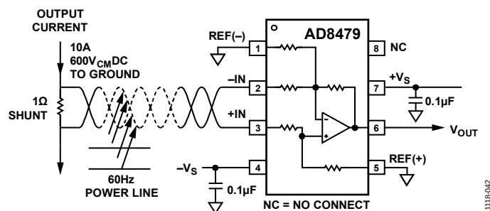
Figure 44. Error Budget Analysis Example: V_{IN} = 10\text{ V Full Scale} , V_{CM} = 600\text{ V DC} , R_{SHUNT} = 1\ \Omega , 1\text{ V p-p} , 60\text{ Hz Power Line Interference}
