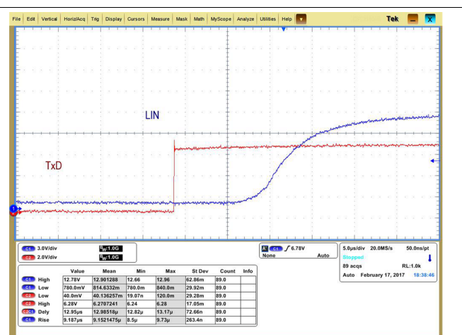
图 32. Recessive to Dominant Propagation
