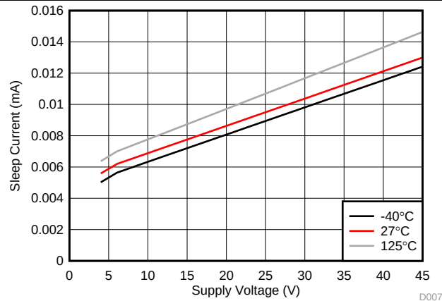
图 7. Sleep Current vs V_{SUP} and Temperature
