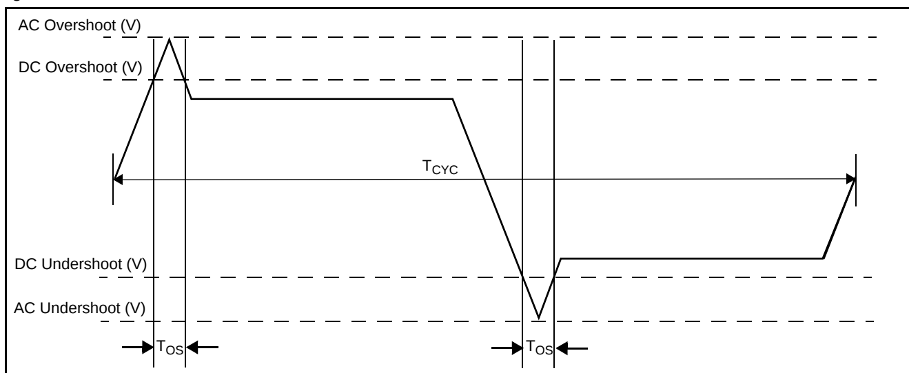
Figure 4. Overshoot Waveform
