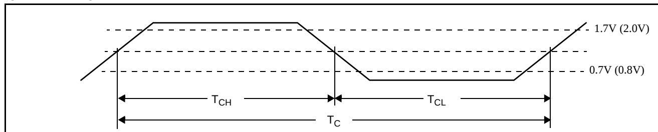
Figure 5. Timing Waveform
