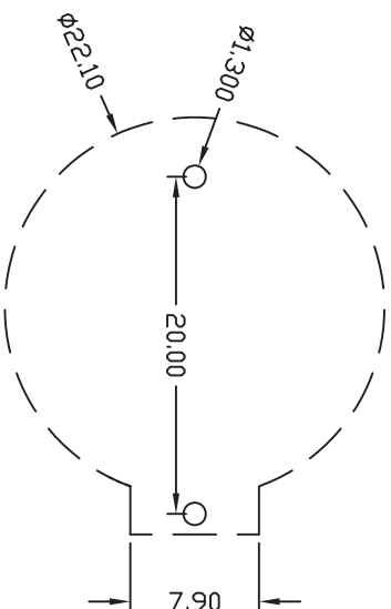
PCB HOLE LAYOUT
