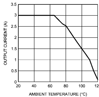
Thermal derating curve V_{IN} = 24\text{V} , V_{OUT} = 5.0\text{V} ,
