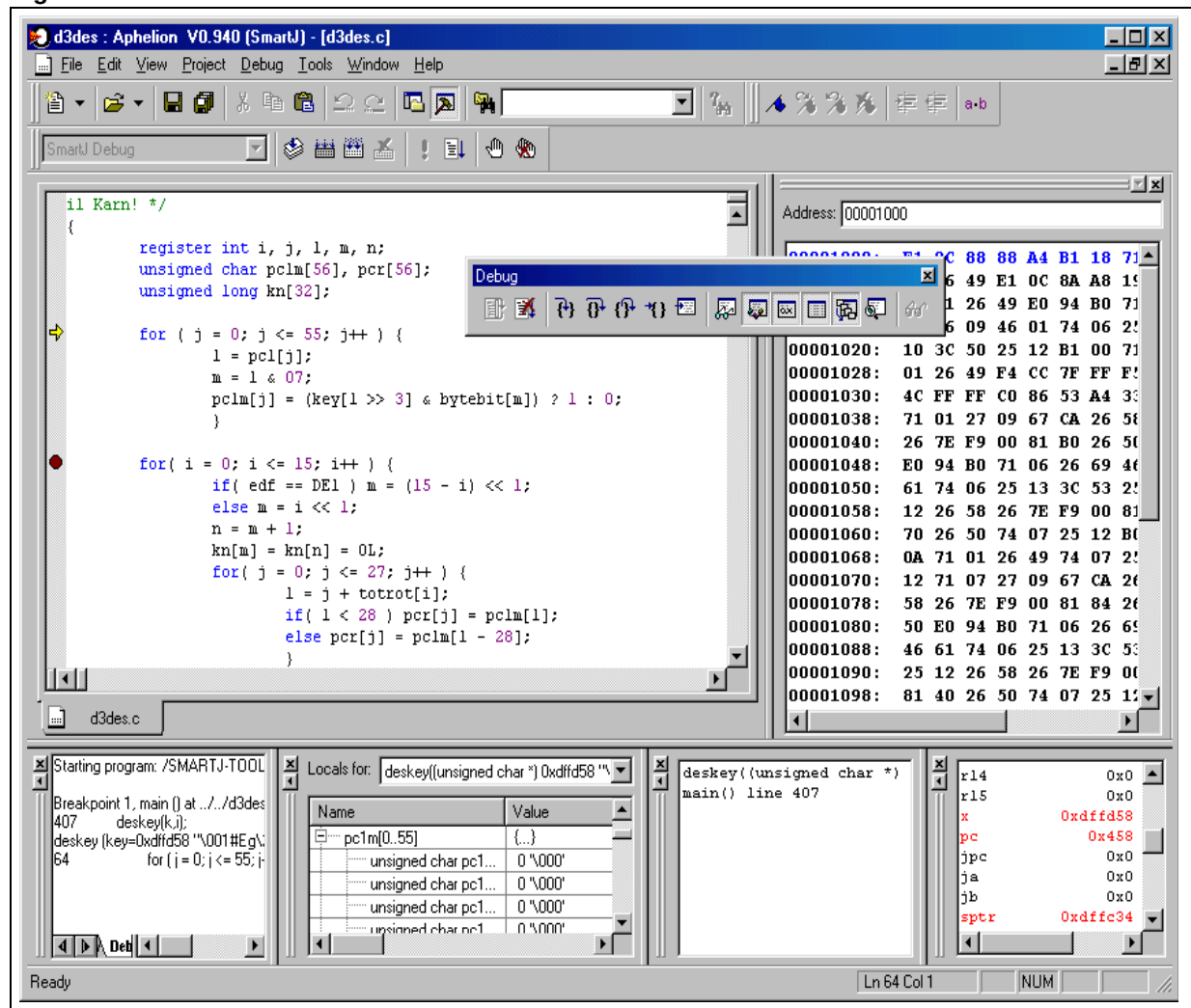
Figure 3. SmartJ™ IDE
