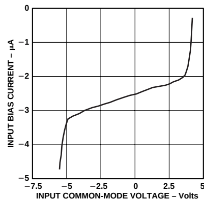
Figure 15. Input Bias Current vs. Input Common-Mode Voltage for \pm 5\text{ V} Supplies
