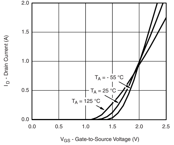
V_{GS} - Gate-to-Source Voltage (V) Transfer Characteristics Curves vs. Temperature
