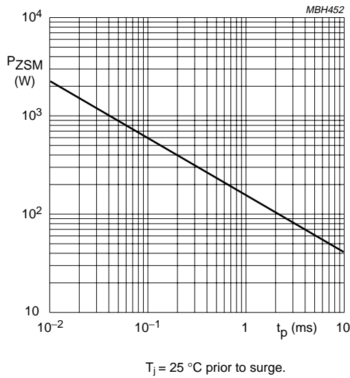
Fig.1 Maximum non-repetitive peak reverse power dissipation as a function of pulse duration (square pulse).
