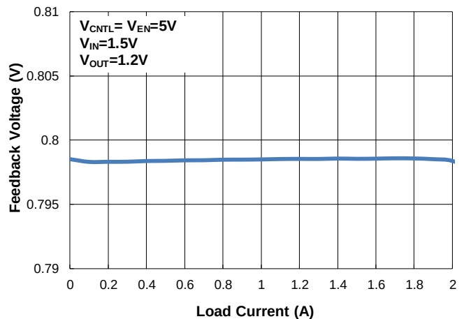
Figure 10. Load Regulation
