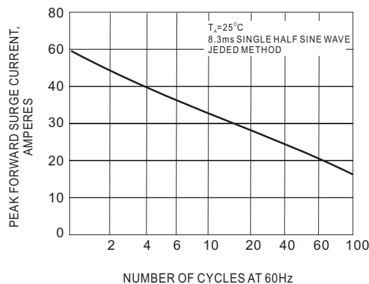
Fig.2 MAXIMUM NON-REPETITIVE PEAK FORWARD CURRENT
