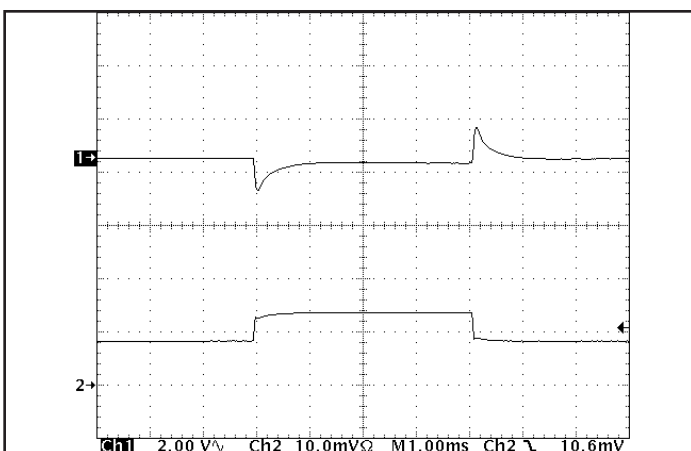
Figure 11: Output voltage response to step-change in load current (50%-75%-50% of Iout(max); dI/dt = 0.1A/μs). Load cap: 100μF, 100 mΩ ESR tantalum cap and 1μF ceramic cap. Ch 1: Vout (2 V/div), Ch 2: Iout (10A/div). Vin = 48V
