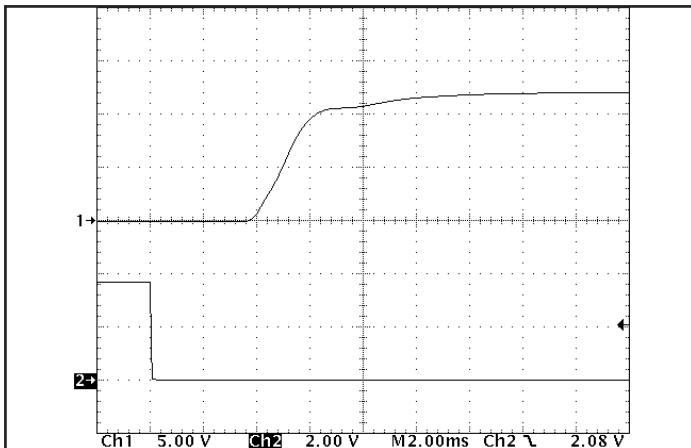
Figure 9: Turn-on transient at half load (resistive load) (2.0 ms/div). Load cap: 3 mF output capacitance. Input voltage pre-applied. Ch 1: Vout (5 V/div), Ch 2: ON/OFF input (2 V/div). Vin = 48V.
