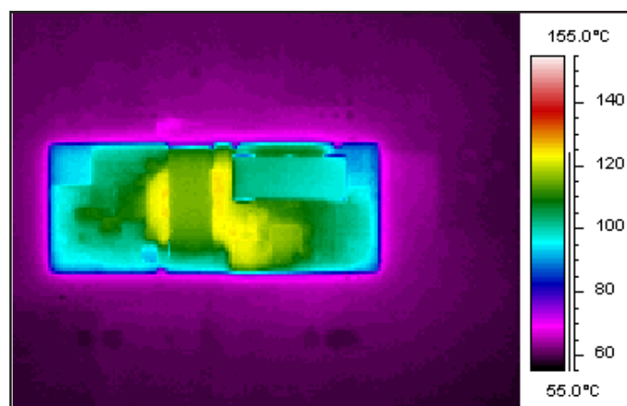
Figure 6: Thermal plot of converter at 14.2 A load current (maximum 125°C derating current) with 55°C air flowing at the rate of 200 LFM. Air is flowing across the converter from pin 3 to pin 1 (nominal input voltage).
