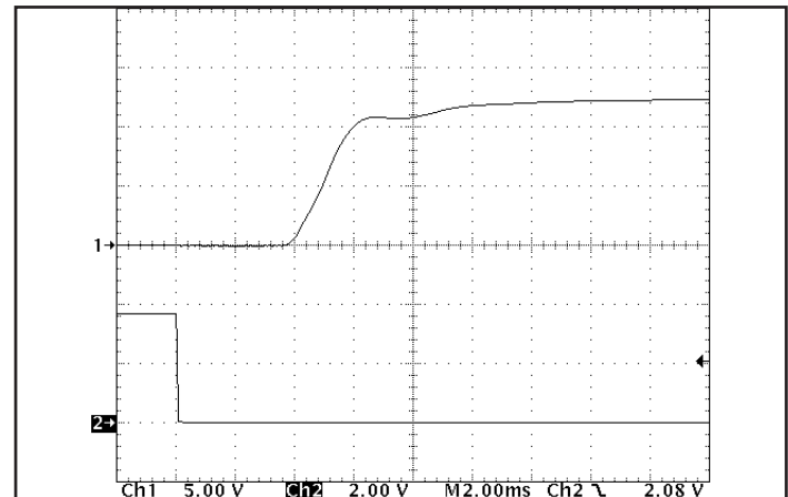
Figure 10: Turn-on transient at zero load (2.0 ms/div). Load cap: 3 mF output capacitance. Input voltage pre-applied. Ch 1: Vout (5 V/div), Ch 2: ON/OFF input (2 V/div). Vin = 48V.
