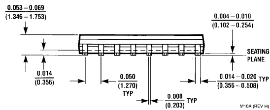
S.O. Package (M) Order Number LM346M NS Package Number M16A
