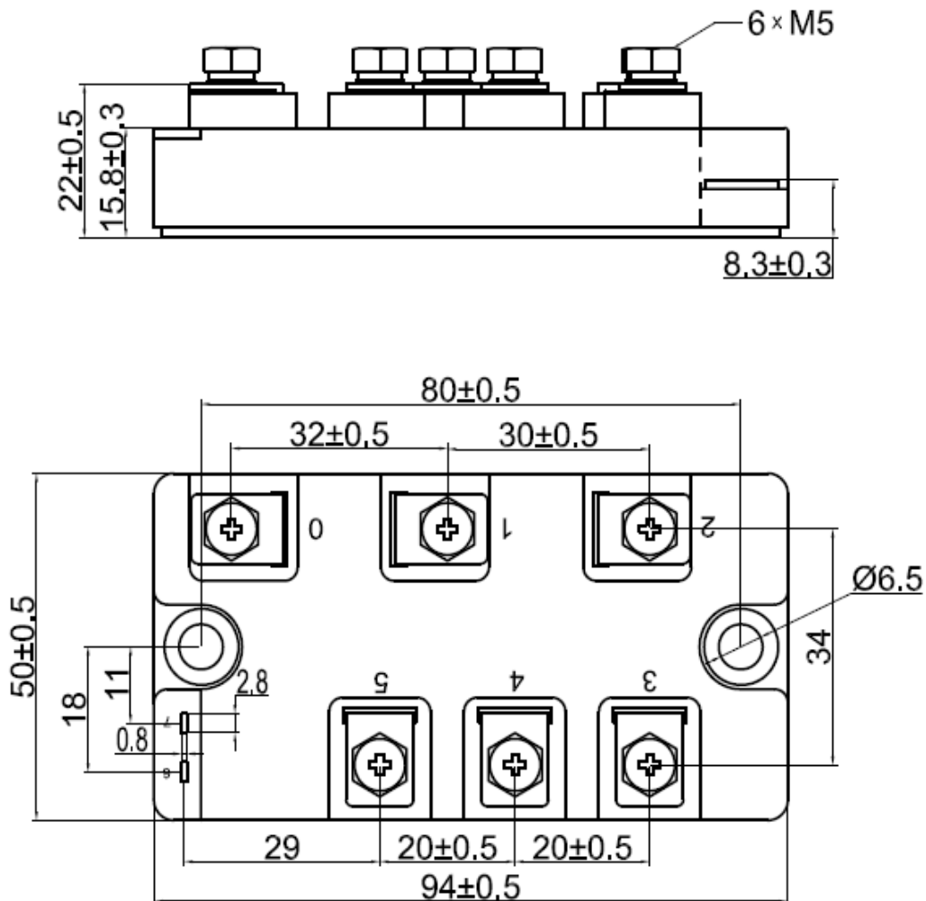
Figure7. Package Outline
