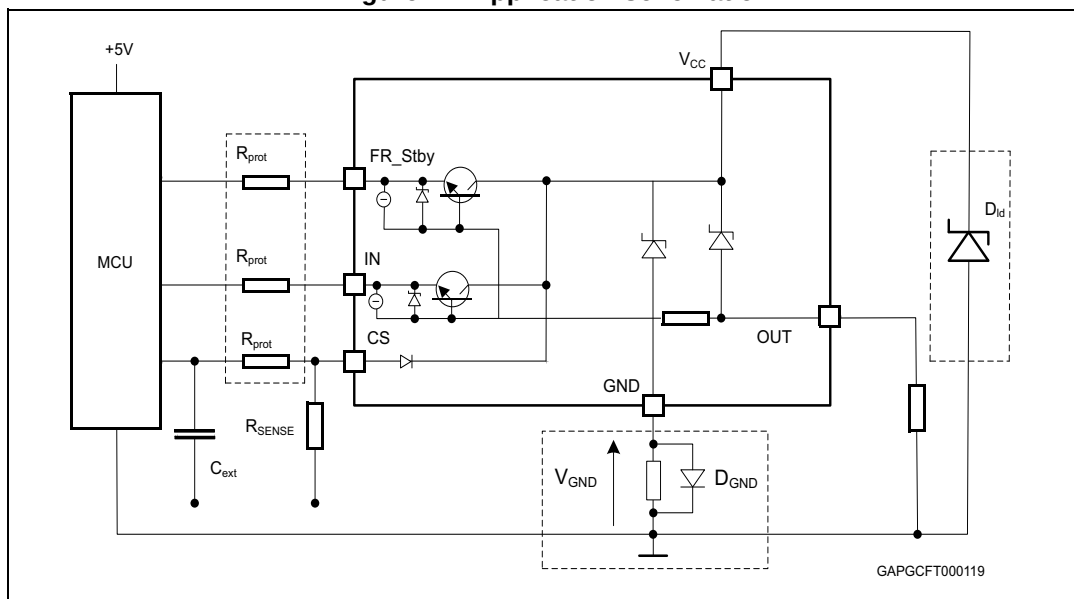
Figure 24. Application schematic
