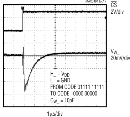
TAP-TO-TAP SWITCHING TRANSIENT (MAX5494/MAX5498)
