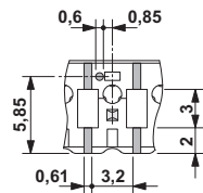
Dimensioned drawing
